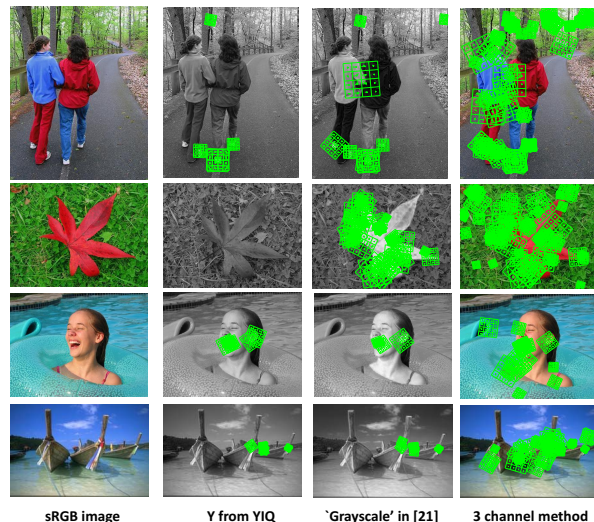
Figure 10. This figure shows several examples of SIFT feature detection. The first column is the color input images. The second and third columns show the results of using Y channel from YIQ and grayscale images obtained from [21], respectively. The last column shows the results by applying SIFT feature detection on three color channels and combining them together.
